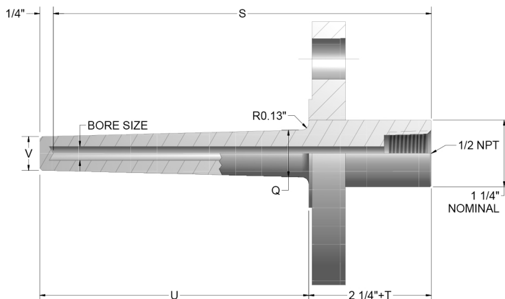
Thermowell Dimensions
