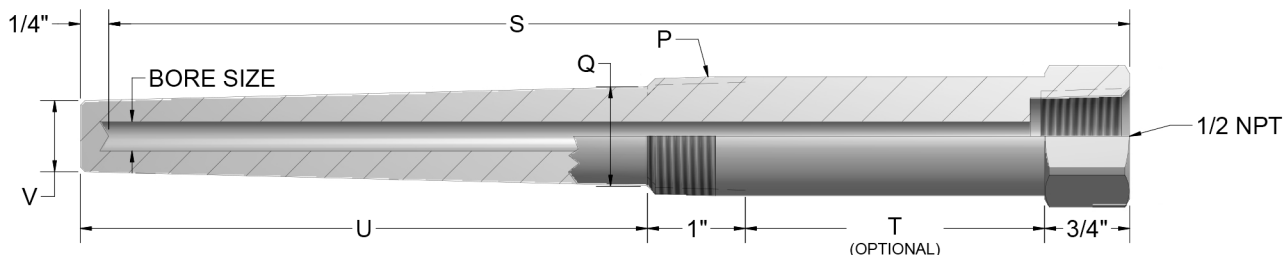
Thermowell Dimensions
