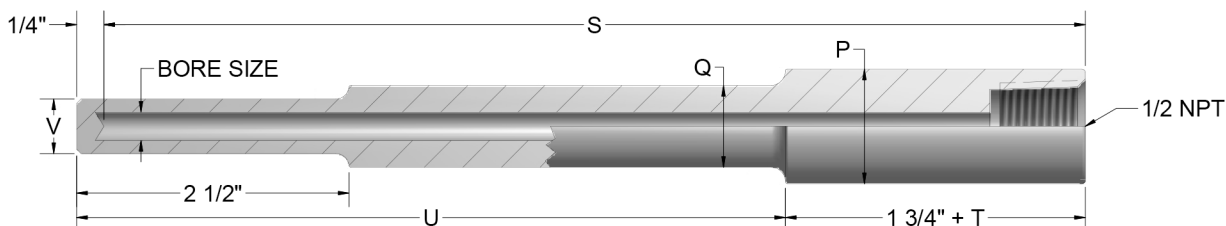
Thermowell Dimensions
