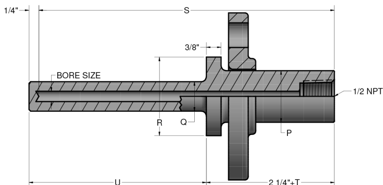
Thermowell Dimensions
